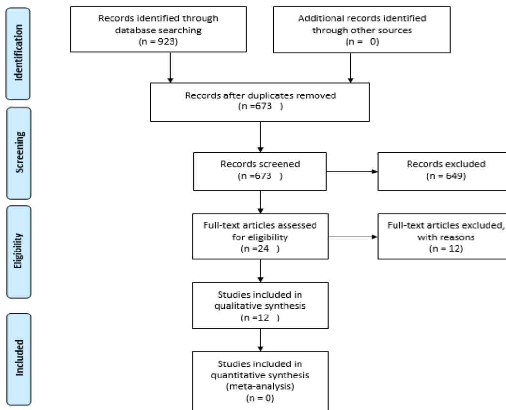
Fig.1: PRISMA flowchart.
